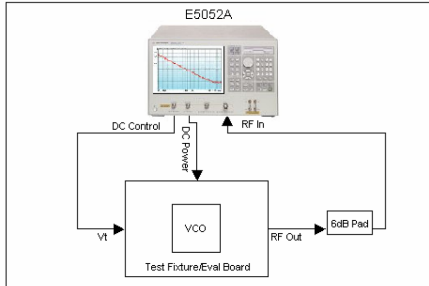
Figure AN-109:1- VCO Phase Noise Measurement Setup
