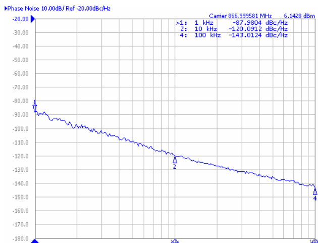
Figure AN-109:2- Phase Noise Plot
