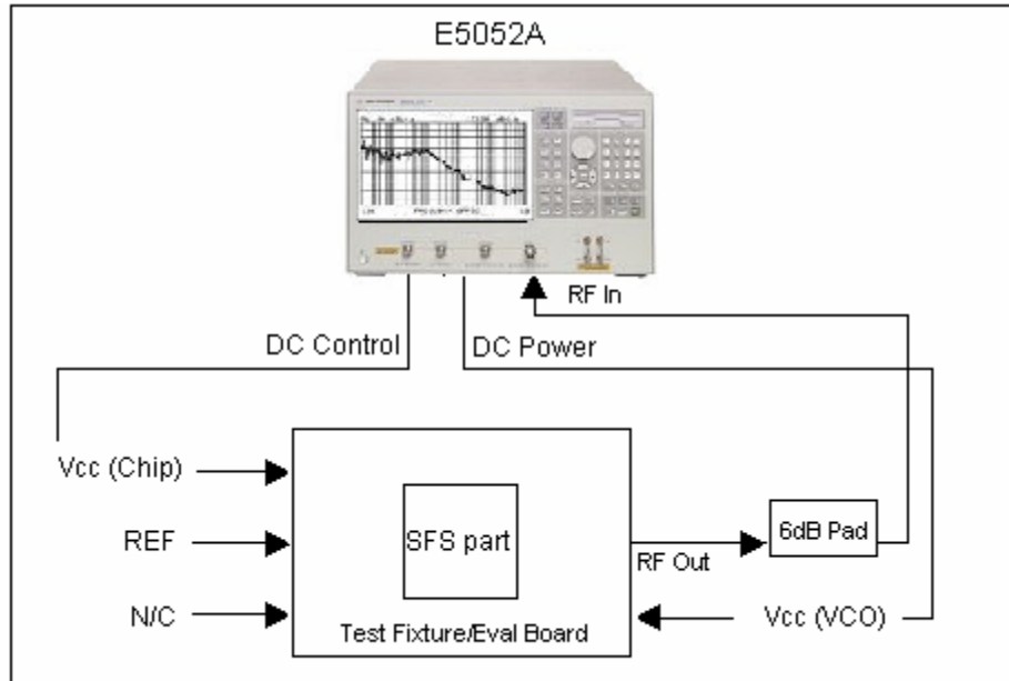
Figure AN-205:1- SFS Series Phase Noise Measurement Setup
