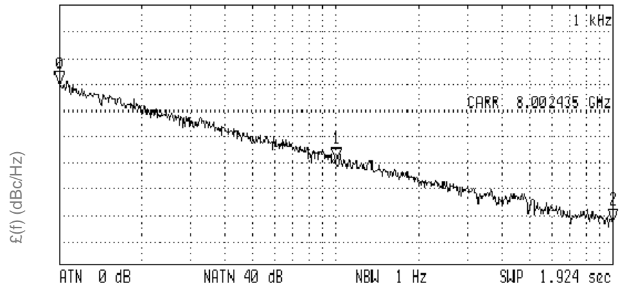
PHASE NOISE (1 Hz BW, typical)
